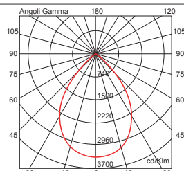
Emissione a fascio largo / Wide beam
