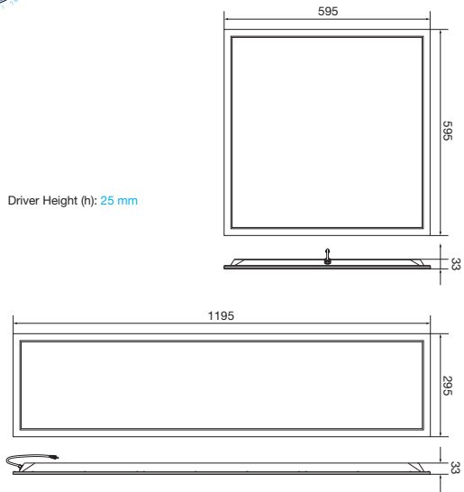
Measures (mm).
