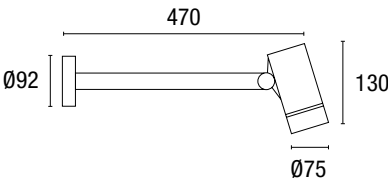
Wall Arm
