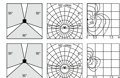
6654.56S.T.-- 35 W QR GY6,35 900 lm 12 V DC vetro trasparente clear diffuser trasformatore remoto SELV non incluso remote SEVL transformer not included
